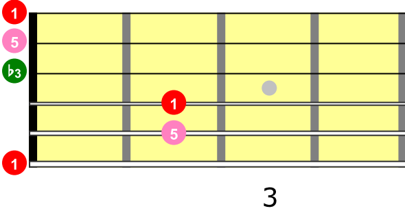
E Minor Triad
