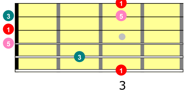
G Major Triad
