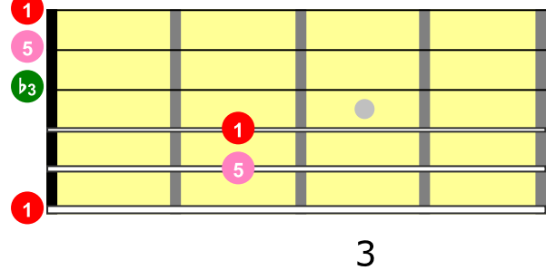
E Minor Triad
