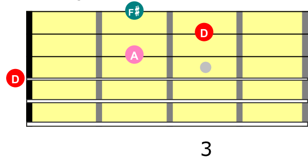
D Major Triad
