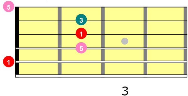
A Major Triad
